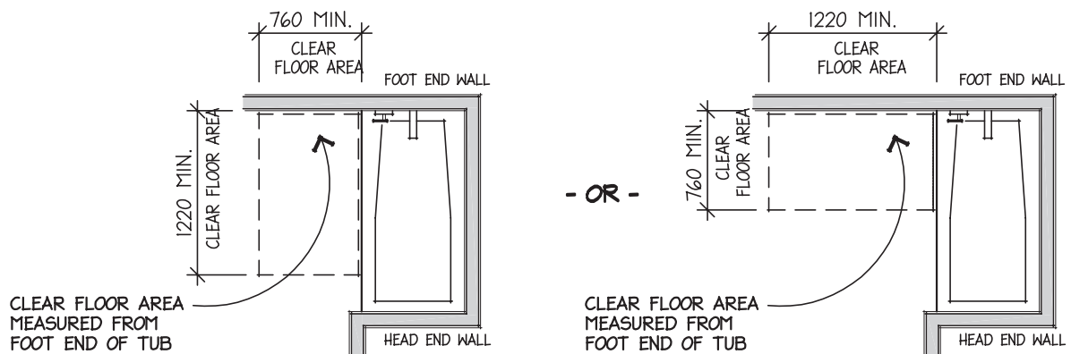
FIGURE 6 CLEAR FLOOR AREA AT TUB
