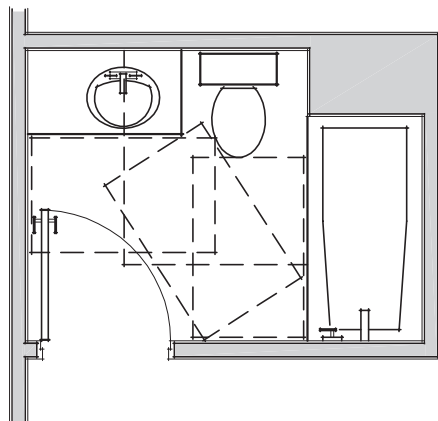
FIGURE 9 EXAMPLES OF BATHROOMS WITH FLOOR AREA TO SUIT "MINIMALLY ACCESSIBLE" REQUIREMENTS
