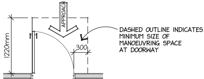
FIGURE 2 FRONT APPROACH, PULL SIDE
