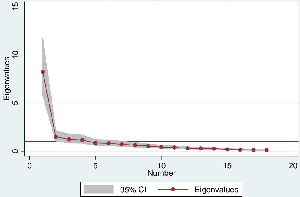
Scree plot of eigenvalues after pca
